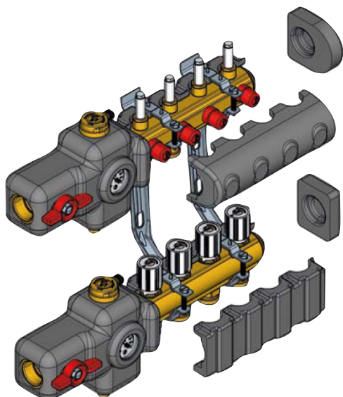
Insulations R553W + R553W-2 + R553F manifold with R554D group + R259D ball valve
